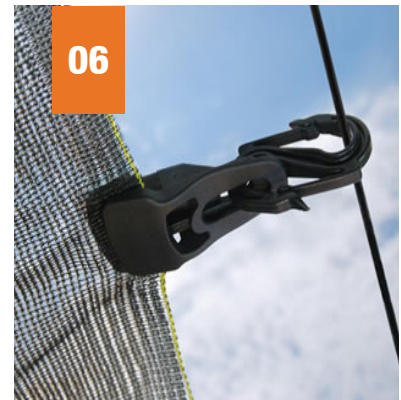
Double hook for anti hail netting
