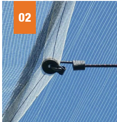
Clips for net fixing
